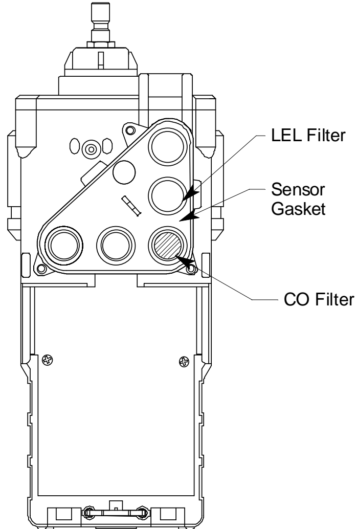
Figure 26: Replacing the LEL and CO Filters
