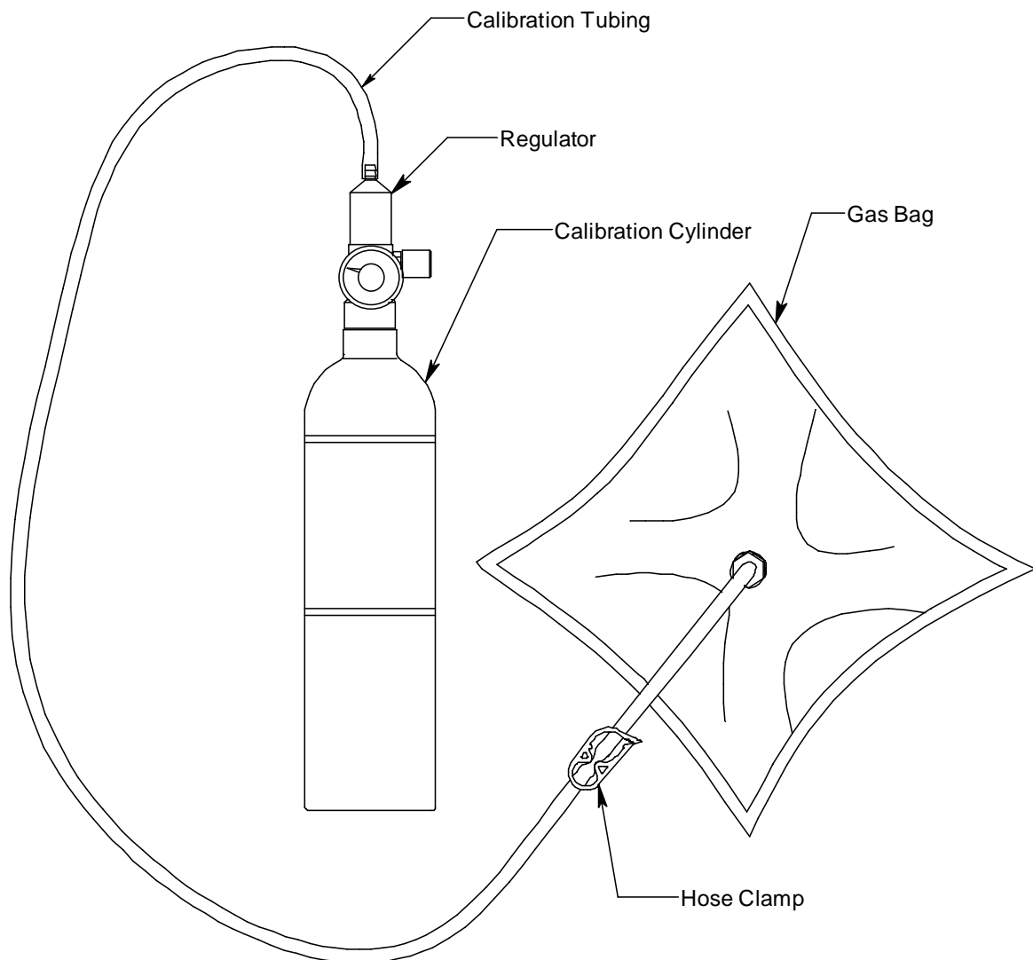
Figure 29: Gas Bag Calibration Kit
