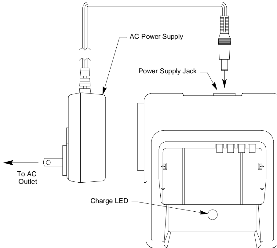
Figure 23: Connecting the Charging Station's AC Adapter
