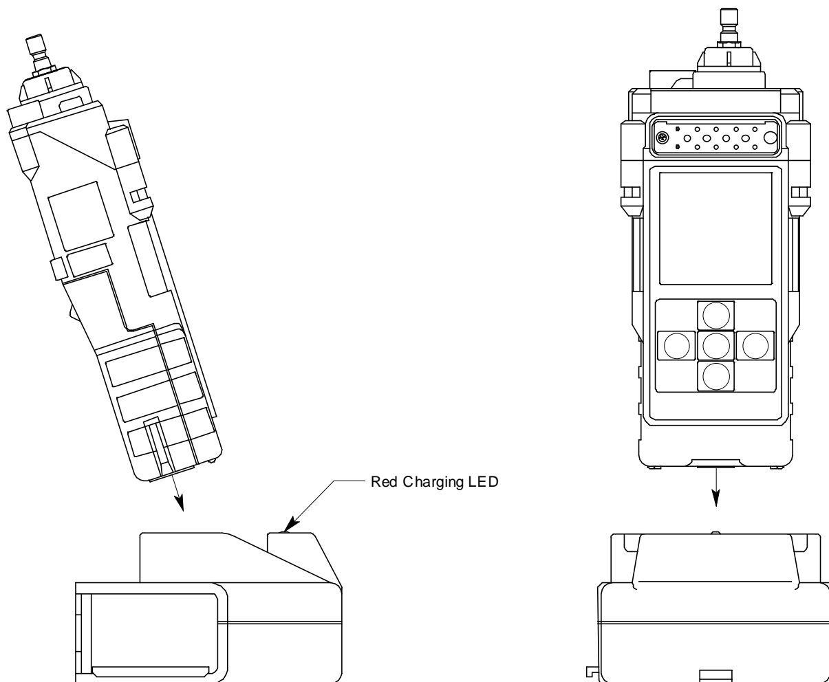
Figure 22: Putting the GX-2012 into the Charging Station
