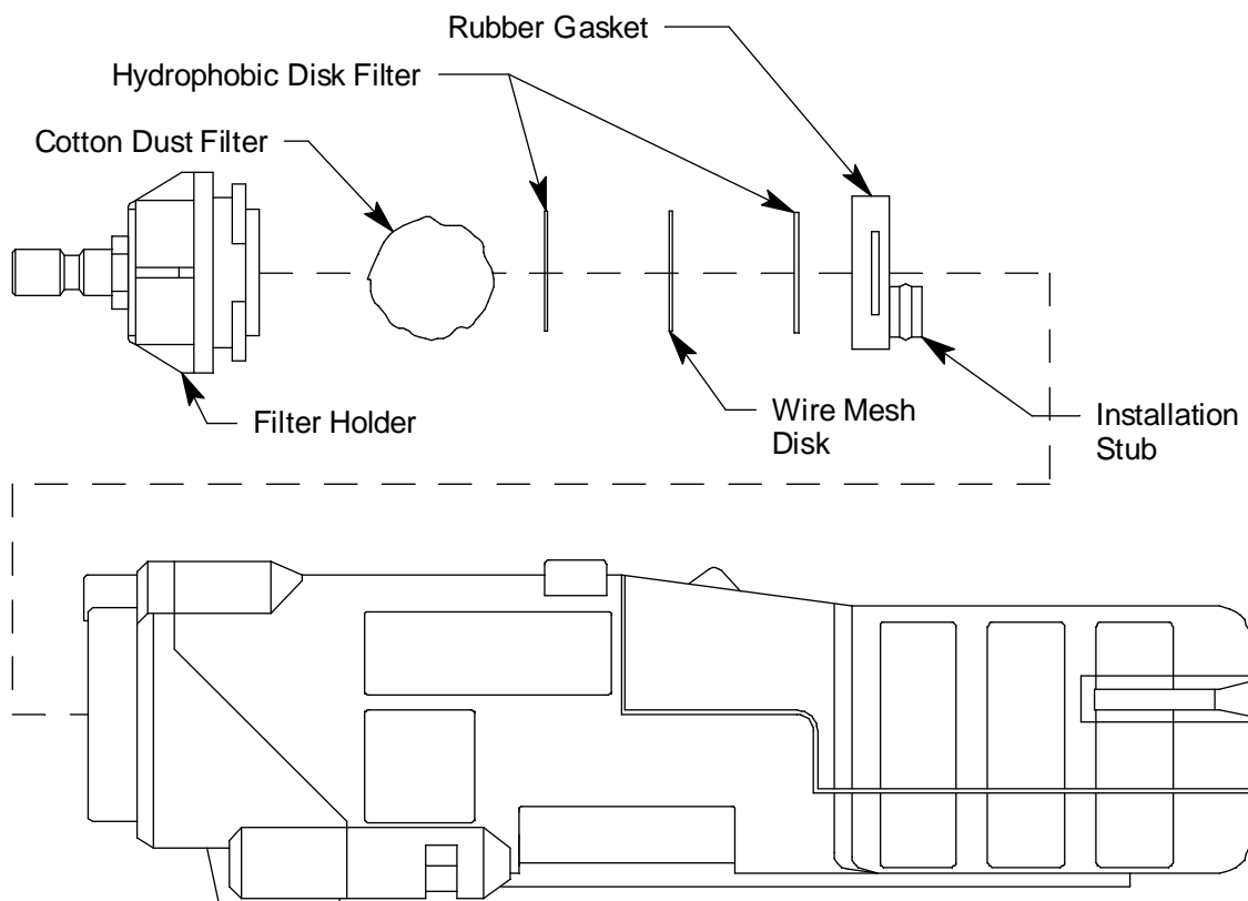
Figure 28: Changing the Filters & Wire Mesh Disk
