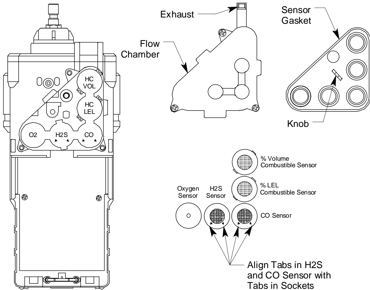
Figure 27: Replacing a Sensor
