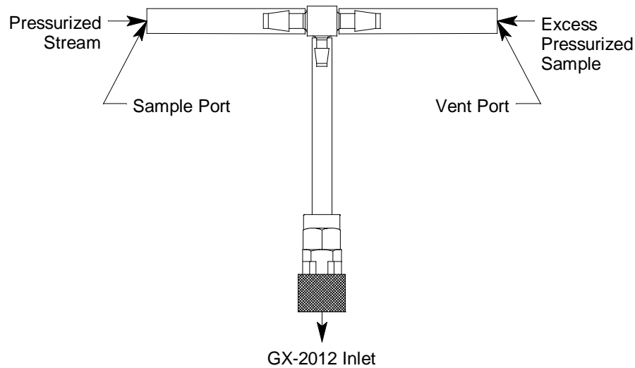
Figure 15: Purge Tee Fitting
