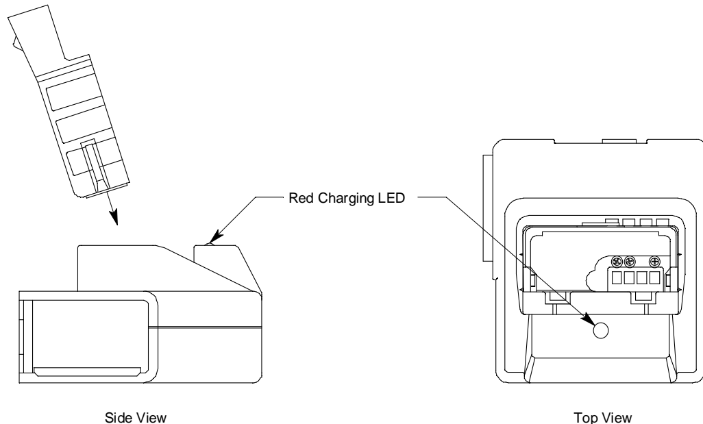
Figure 25: Putting the Battery Pack into the Charging Station
